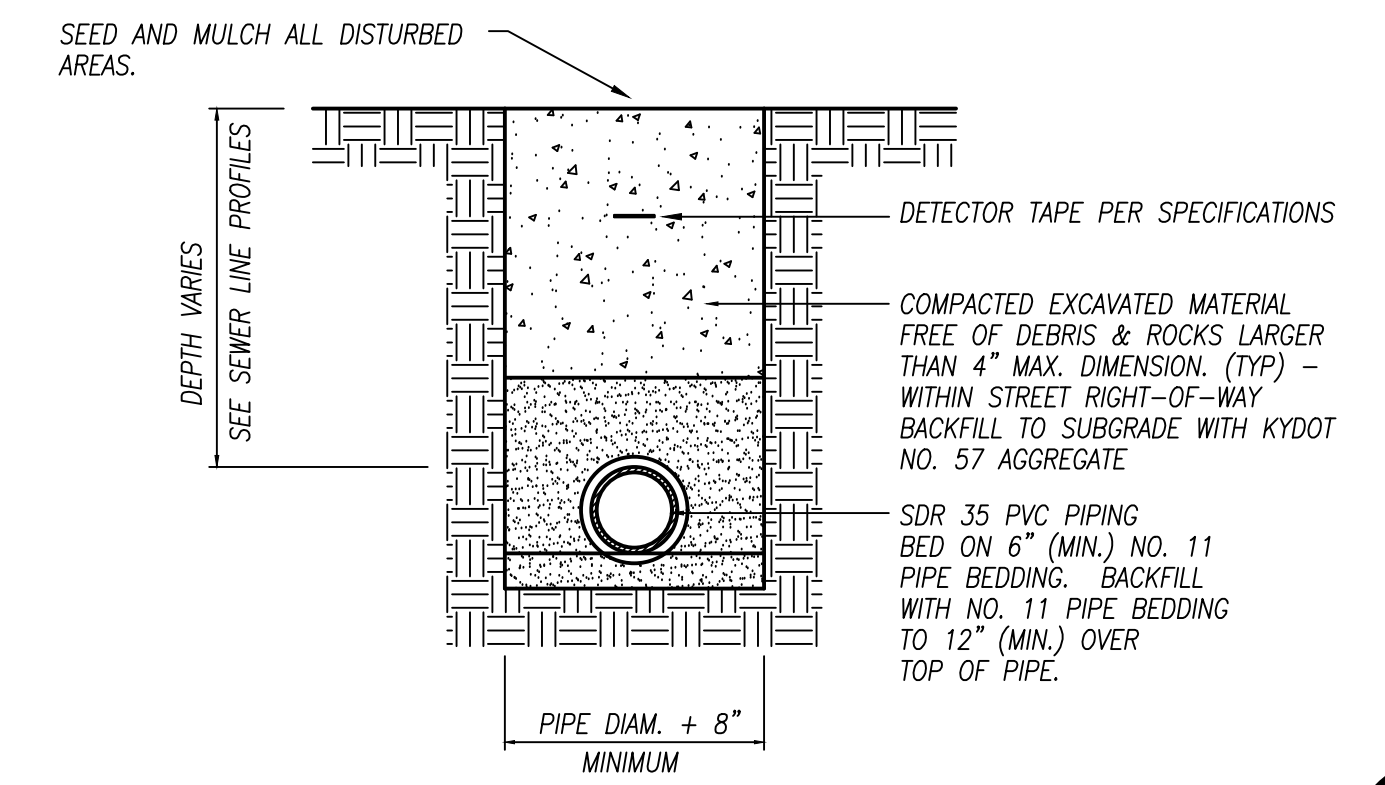
SEWER MAIN BEDDING & BACKFILL-OPEN CUT 8 D1 NOT TO SCALE
