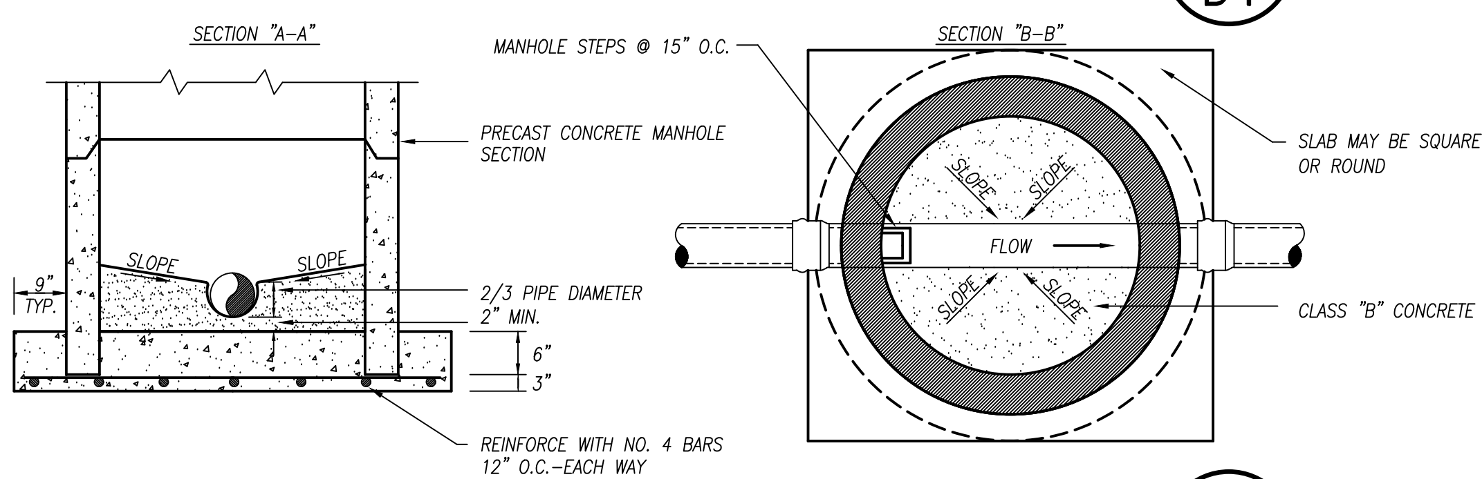
TYPICAL MANHOLE SECTIONS 2 D1 NOT TO SCALE
