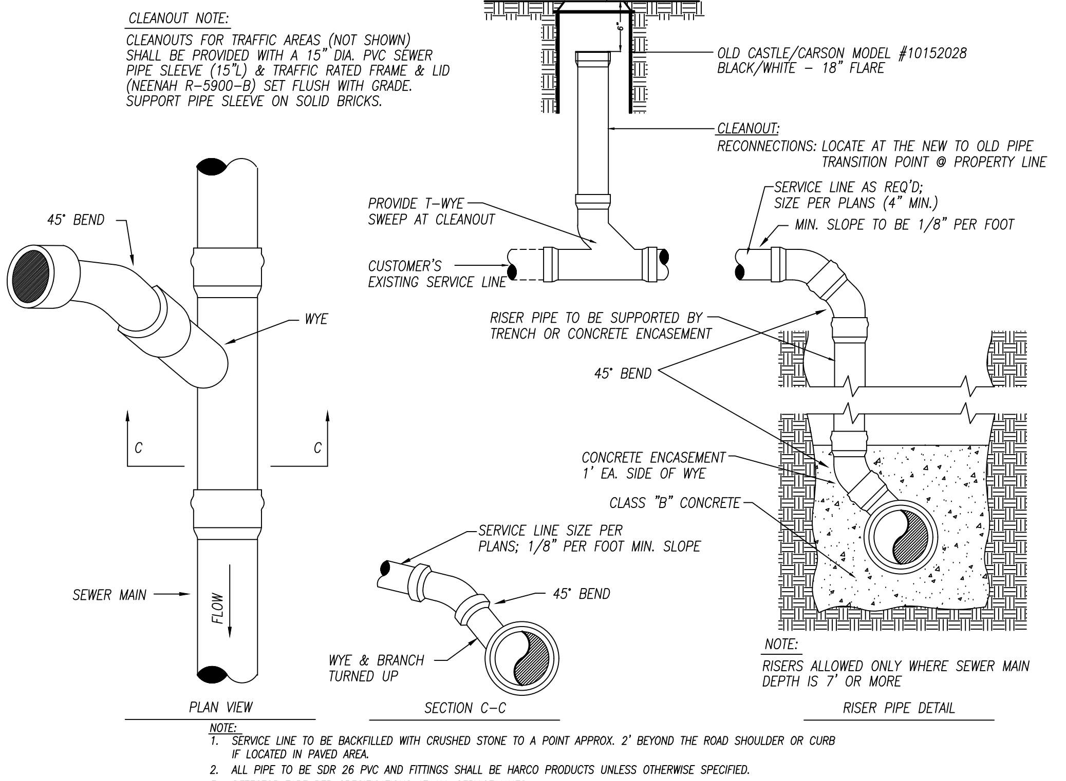
SERVICE CONNECTION: OPEN CUT OR BORED 3 D1 NOT TO SCALE
