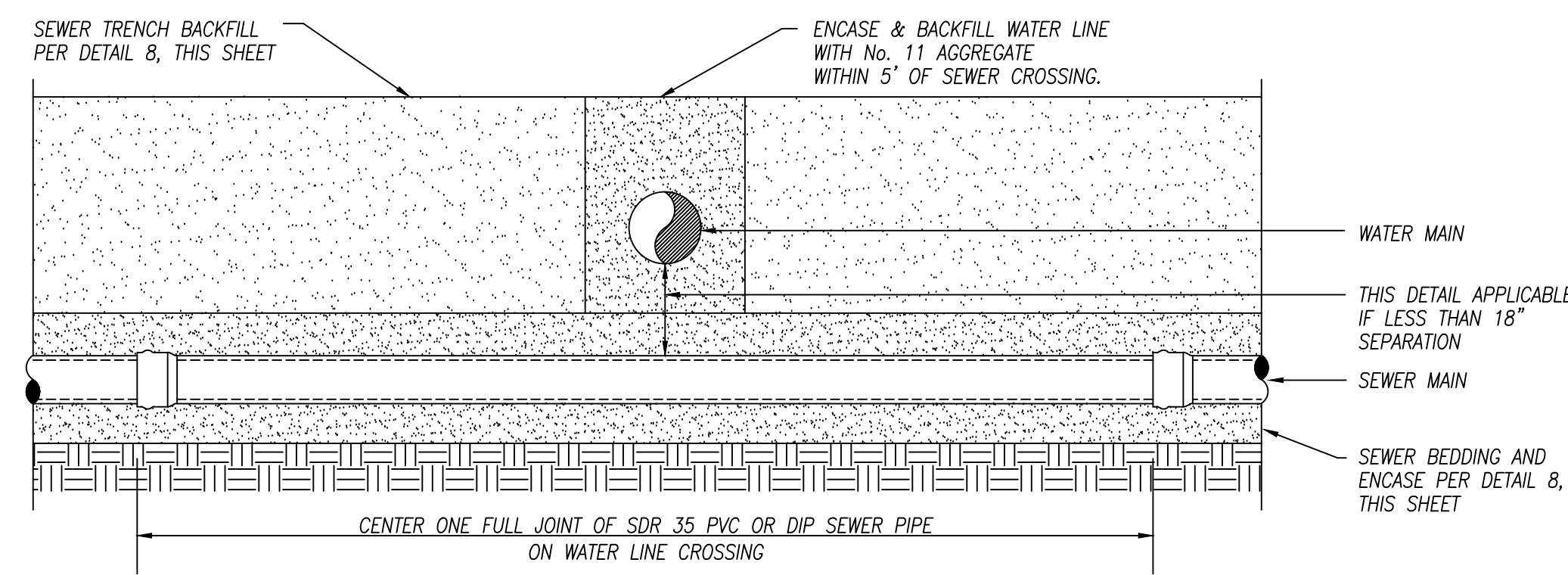
WATER LINE CROSSING 7 D1 NOT TO SCALE
