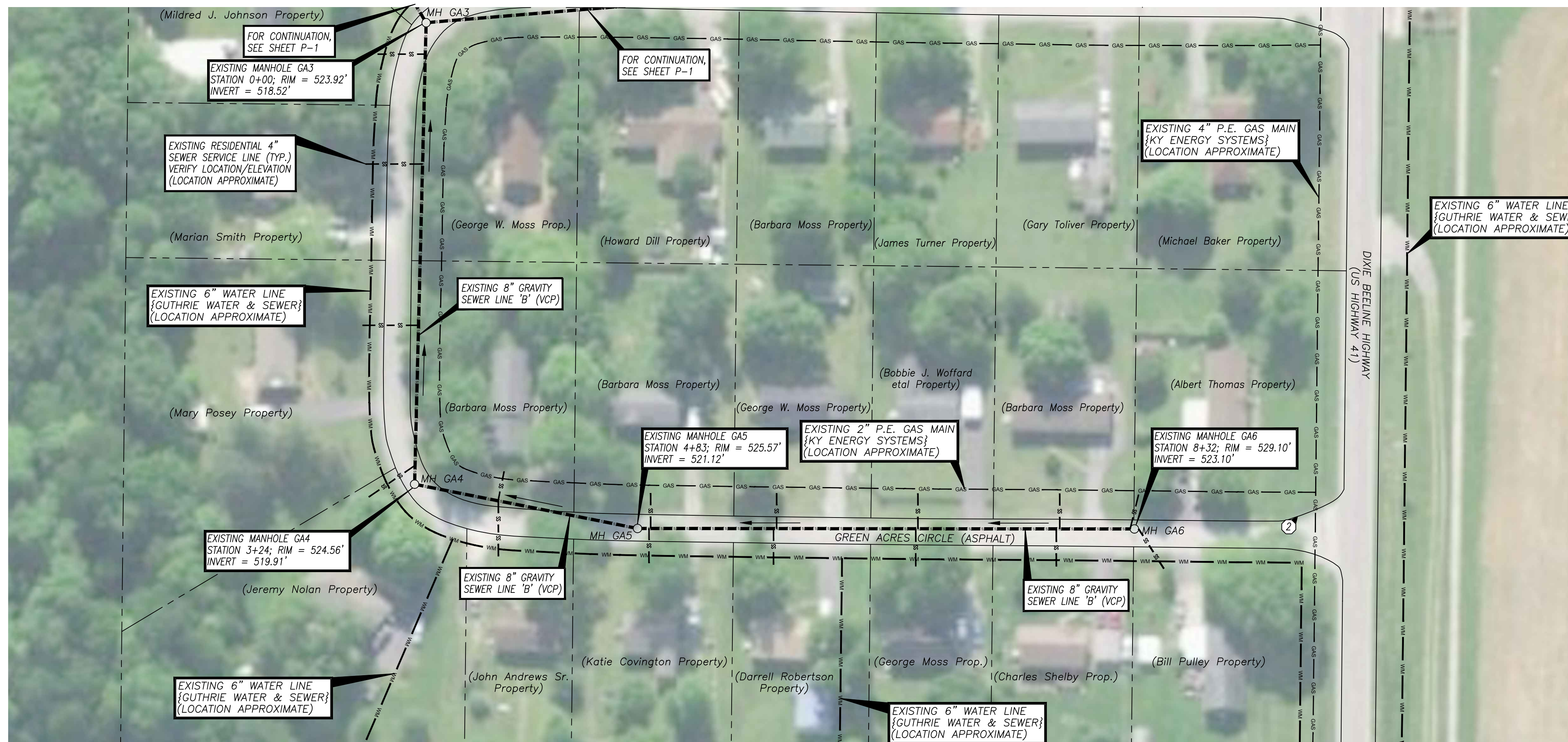
EXISTING GRAVITY SEWER MAIN 'LINE B' PLAN: MANHOLE GA3 TO MANHOLE GA6
