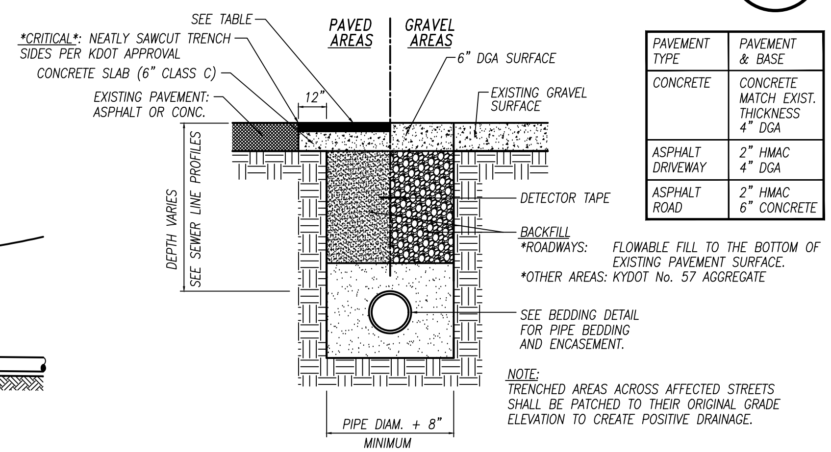
PAVEMENT REPAIR/REPLACEMENT (SEWER) 9 D1 NOT TO SCALE
