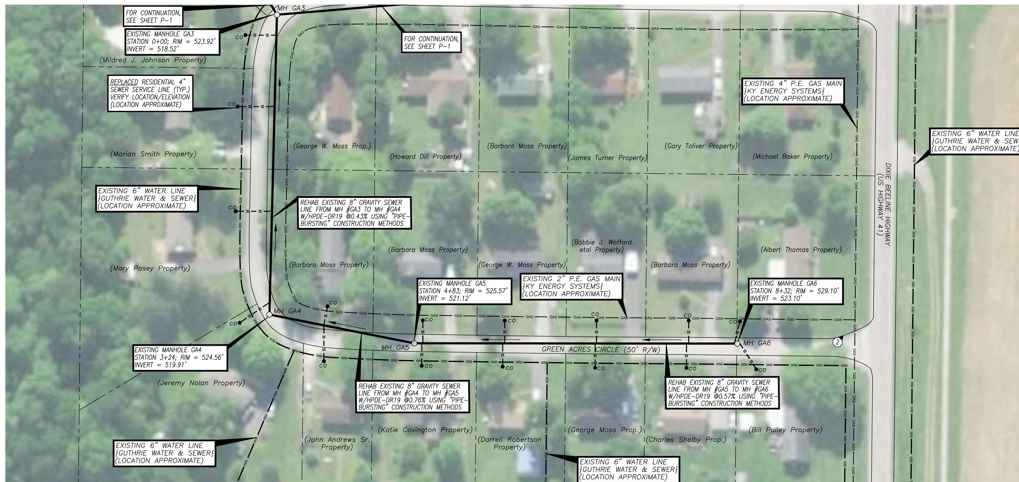
PROPOSED GRAVITY SEWER MAIN 'LINE B' PLAN: MANHOLE GA3 TO MANHOLE GA6
