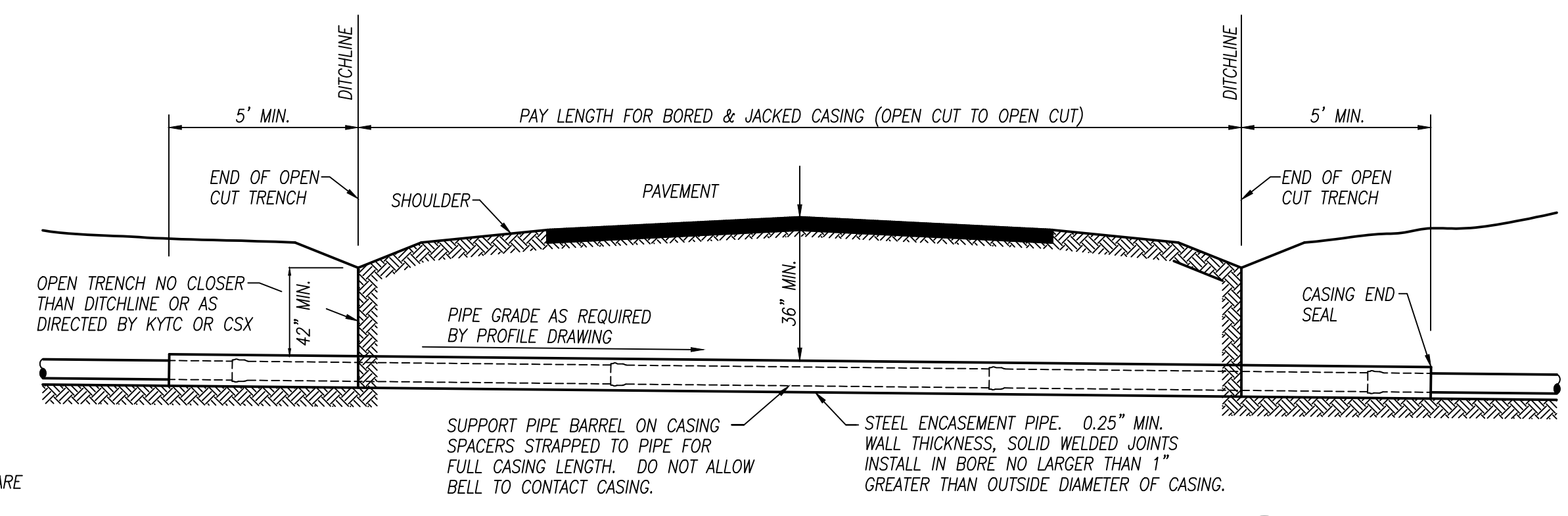
STEEL CASED ROAD BORE-SEWER 5 D1 NOT TO SCALE
