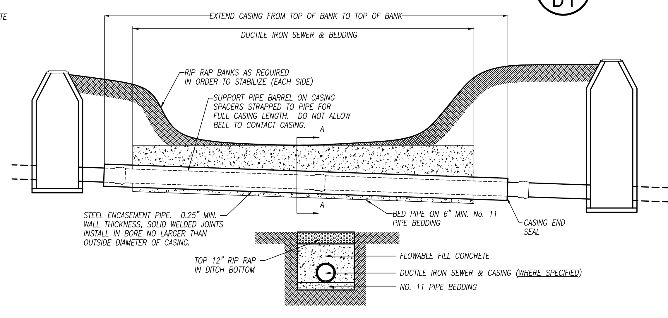
WIDE STREAM CROSSING - OPEN CUT 6 D1 NOT TO SCALE
