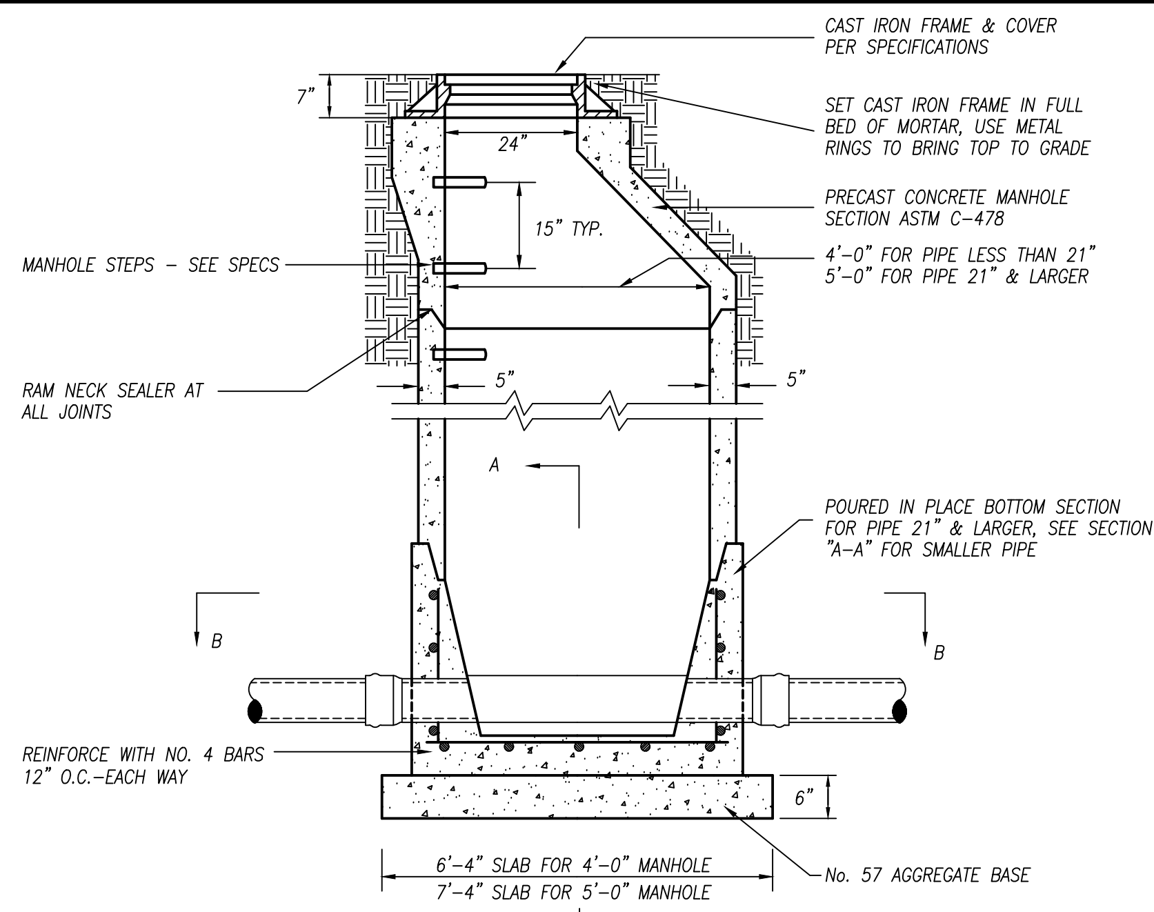
TYPICAL MANHOLE 1 D1 NOT TO SCALE
