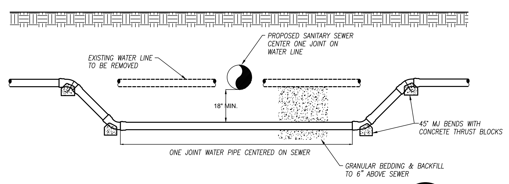
WATER LINE LOWERING NEW SEWER CROSSING 4 D1 NOT TO SCALE
