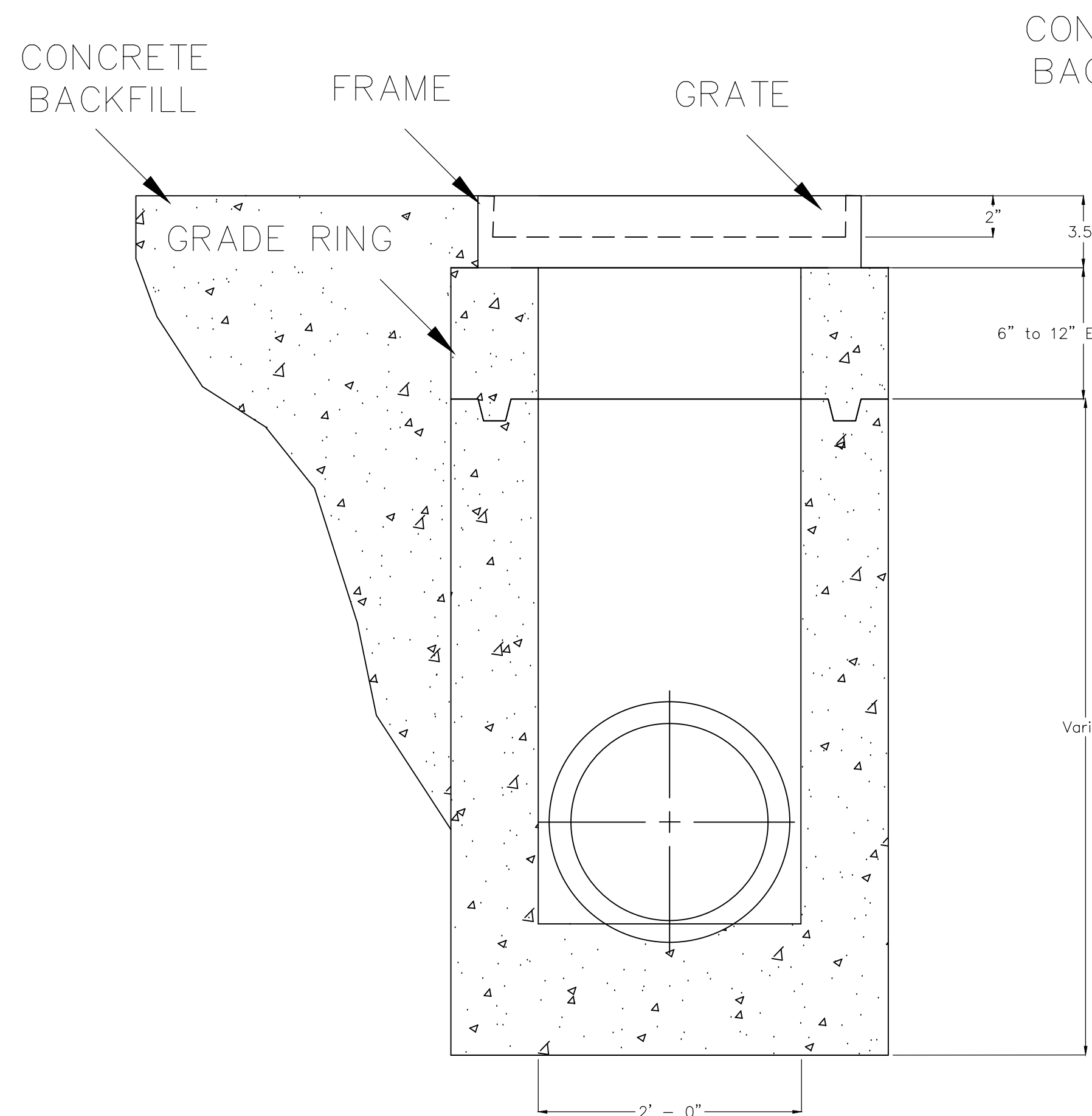
PRECAST BOX SECTION ROAD VIEW
