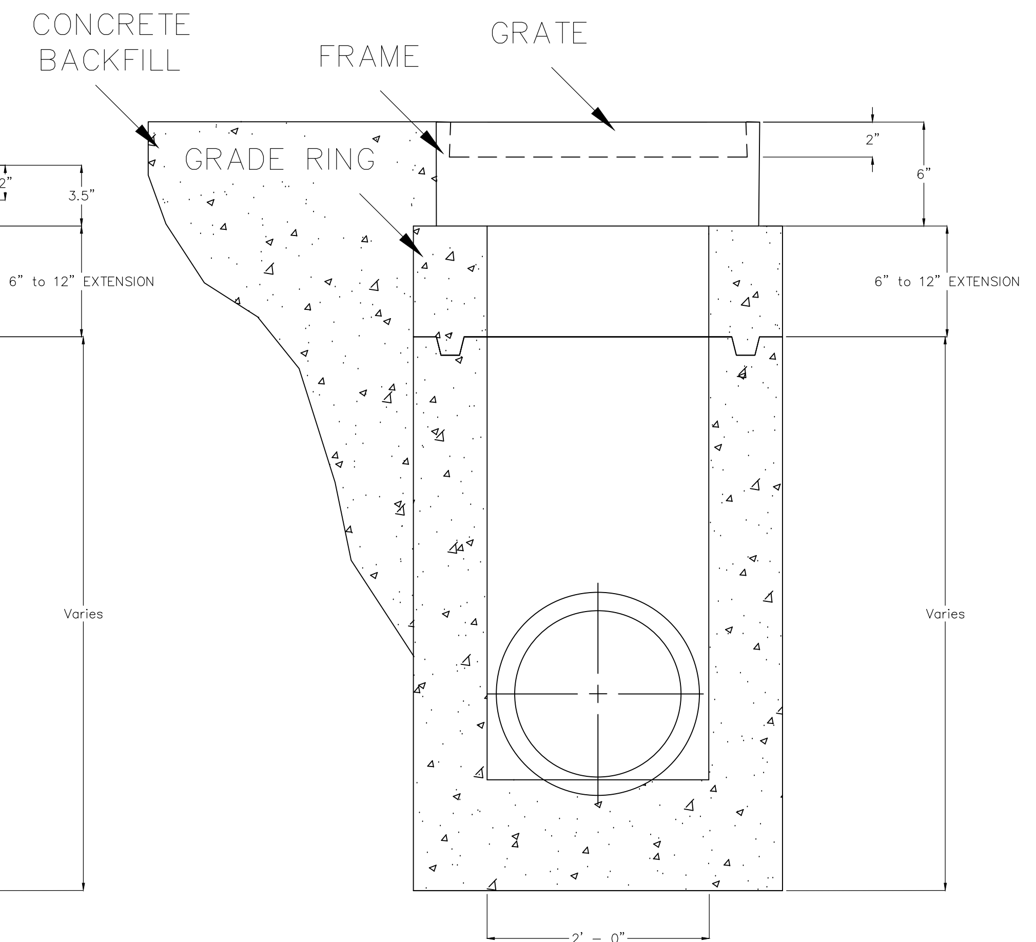
PRECAST BOX SECTION CURB VIEW
